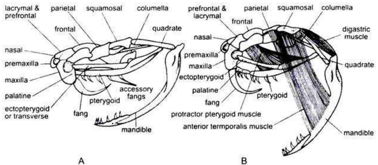
Fig. 23.4. Skull of a viper showing biting mechanism. A–Mouth closed at rest; B–Mouth opened when striking the prey.
