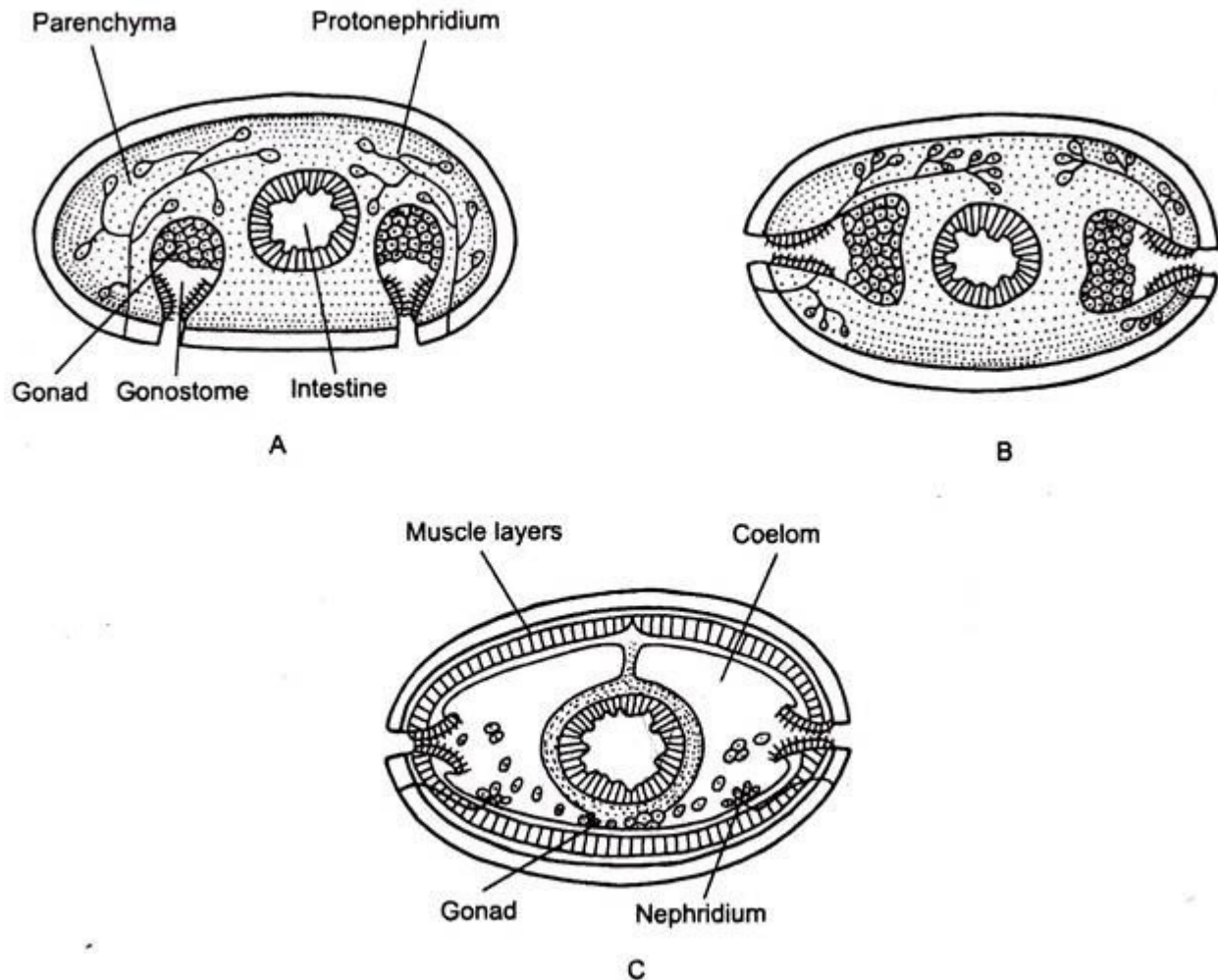
Fig. 17.53: Diagrams showing the gonocoel theory of coelom formation.
